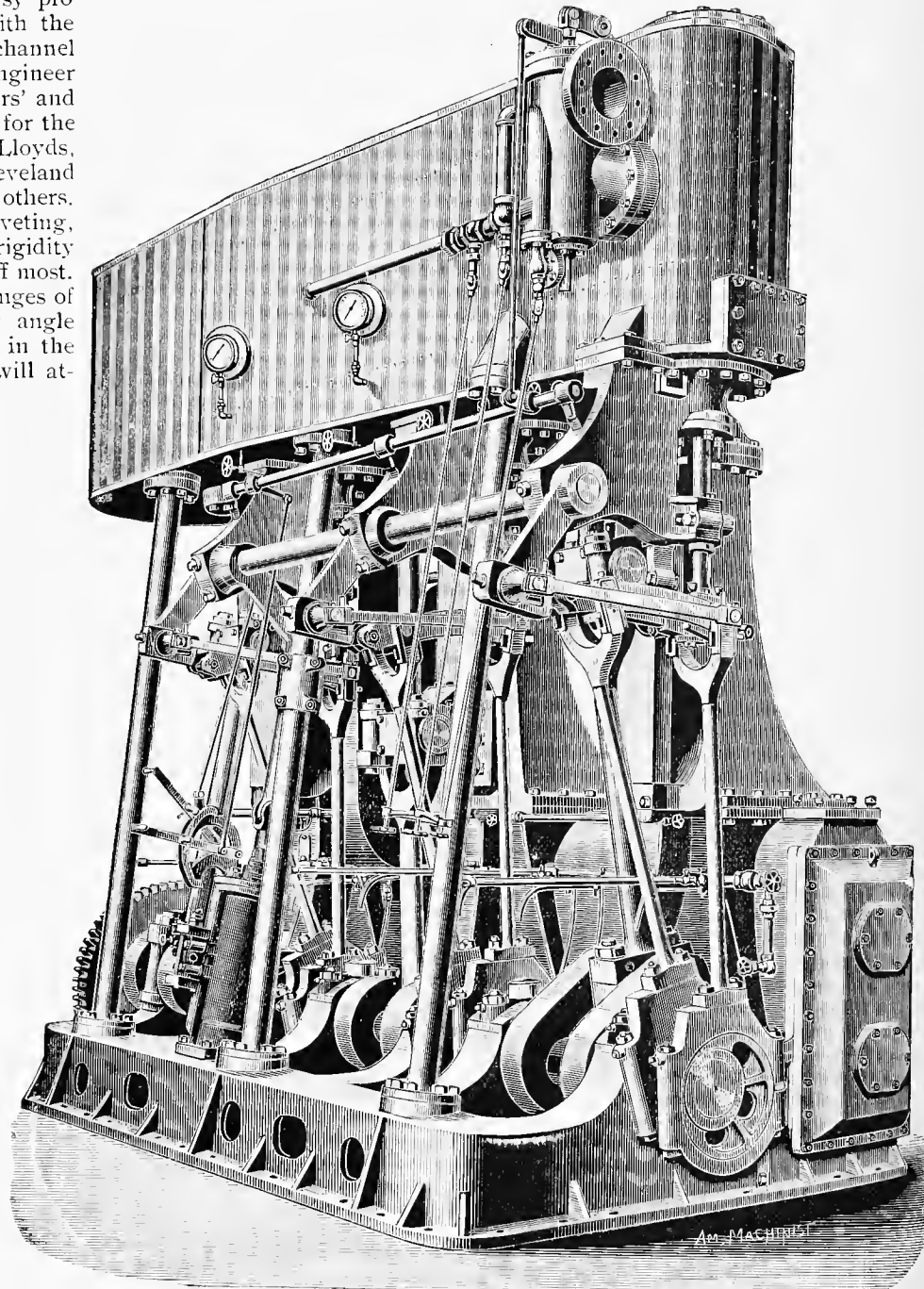
TRIPLE-EXPANSION ENGINE OF THE BRIDGEPORT LINE STEAMER NUTMEG STATE.
